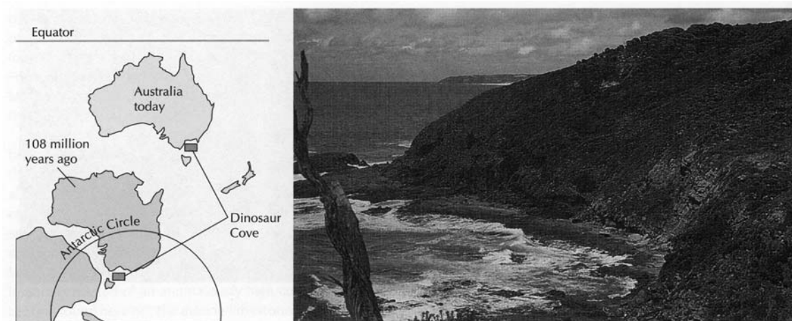
figure 5.10 Dinosaur Cove in Australia has produced fossils of dinosaurs that lived on the continent about 100 million years ago when Australia occupied a position much nearer the South Pole than it does today. (from Rich, P. and T. H. Rich, July 1993, Australia's pluar dinosaurs, Sci. American, p. 52)
