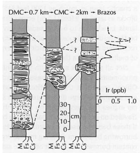
figure 5.19 Diagram illustrating the layers of rock spanning the K-T boundary along the Brazos River in Texas. Note the large blocks at the base of each section. These are interpreted to have been ripped up by a tsunami generated by the Chicxulub impact.
