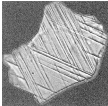
figure 5.14 This photograph of a quartz crystal from the boundary clay in Wyoming was taken under a microscope. Although it is less than one mm in length, it shows the multiple planes of fracturing that most scientists believe resulted from the impact near present-day Yucatan. (from Bohor, B. F., 1990, Shocked quartz and more; impact signatures in Cretaceous/Tertiary boundary clays, Geol. Soc. Am., Sp. Pap., 247, p. 336)
