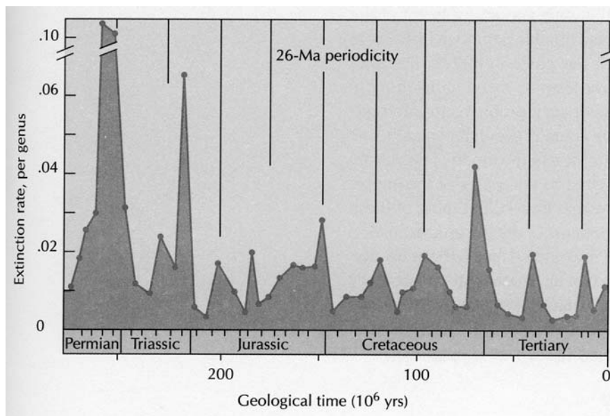
figure 5.19 The peaks on this graph document the episodes of mass extinction in the geologic past. (from Hallam, A., 1989, Catastrophism in geology , In Alvarez, W., et al., Catstrophes and Evolution: Astronomical Foundations , Cambridge Univ. Press, Cambridge, p. 37)
