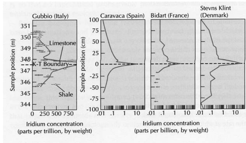
figure 5.06 These charts illustrate the elevated levels of iridium found at four different sites spanning the K-T boundary. Such "anomalous" concentrations of iridium have now been found at over 100 sites around the world. (from Courtillot, V., October 1990, A volcanic eruption, Sci. American, p. 91)
