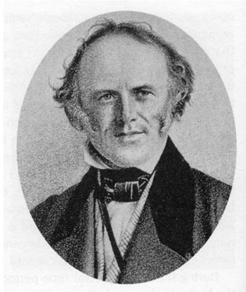
figure 5.03 Charles Lyell, often acknowledged as the father of modern geology, laid out the detailed geological evidence supporting uniformitarianism in his book entitled Principles of Geology .
