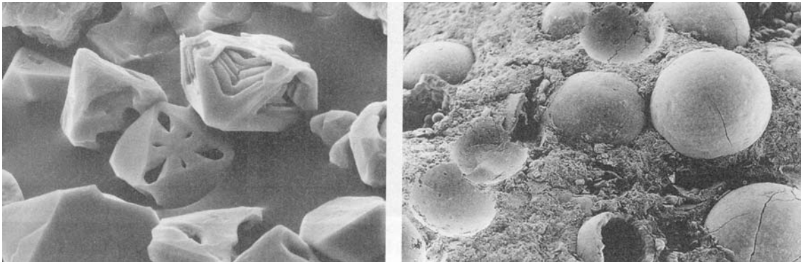
figure 5.16 (left) This scanning electron microscope photos of spinel crystals from the boundary clay at Caravaca, Spain is thought by many scientists to represent evidence for impact. (from Bohor, B. F., 1990, Shocked quartz and more; impact signatures in Cretaceous/Tertiary boundary clays, Geol. Soc. Am., Sp. Pap., 247, fig. 3).
