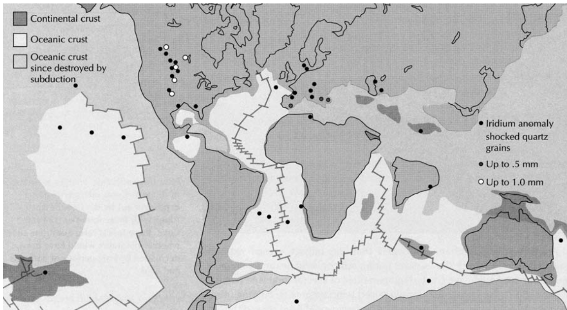
figure 5.11 This map illustrates the global distribution of geological evidence used to support the impact hypothesis for dinosaur extinction. (from Alvarez, W. and F. Asaro, October 1990, An extraterrestrial impact, Scientific American, p. 79)
