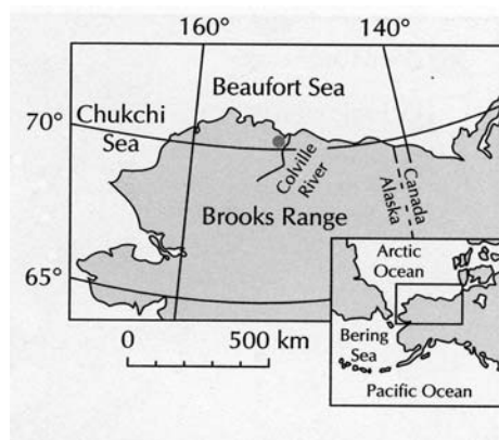
figure 5.11 Near the north Pole, another assemblage of dinosaurs has been uncovered along exposures cut by the Colville River. Along with those found at Dinosaur cove, these fossils raise questions about whether dinosaurs would have been decimated by long periods of darkness and cold. (from Clemens, W. A. and L. G. Nelms, 1993, Paleocological implications of Alaskan terrestrial vertebrate fauna in the latest Cretaceous time at high paleolatitudes, Geology , v. 21, pp. 503-506.
