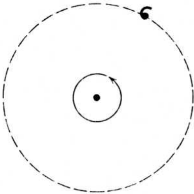
Rotation 360^\circ 1
