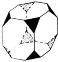
Octahedron {111}
