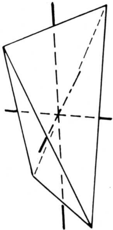
\{hk\} + Disphenoid
