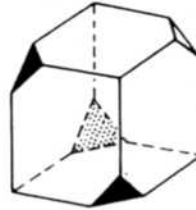
-Tetrahedron {111}
