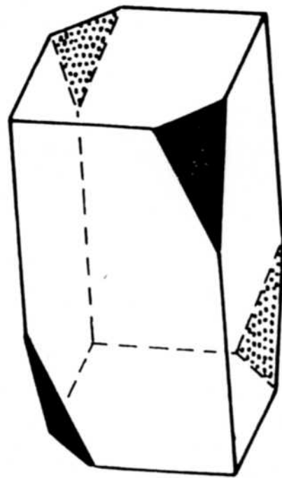
\{hk\} + Disphenoid modifying a tetragonal crystal
