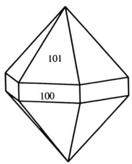
\beta -Quartz
