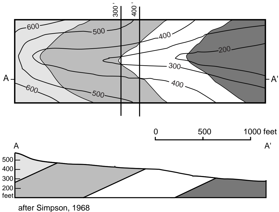
Figure 4. Geological map and cross section of 4 units that strike N-S and dip W. 300' and 400' foot strike lines for the upper contact of the white unit are shown. The 300' strike line is W of the 400' strike line, as it must be if the units dip W. Parallel strike lines with the same spacing could also be drawn for the upper contact of the dark gray unit (at 200' and 300') and the medium gray unit at (400' and 500'), indicating that all contacts are planar and parallel.
