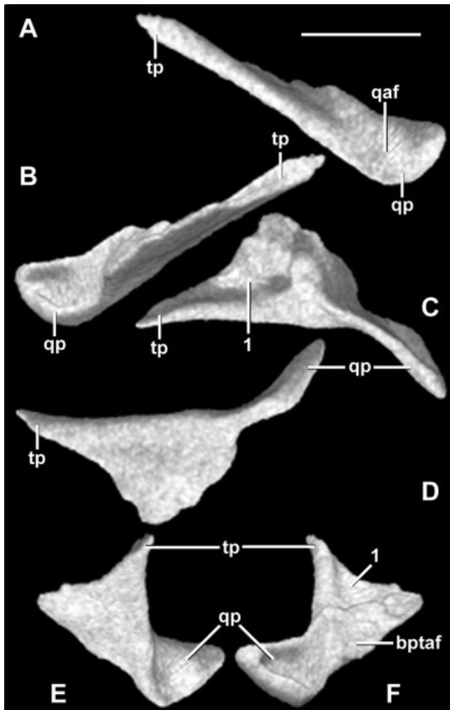
Fig. 13. Left pterygoid in (A) lateral, (B) medial, (C) dorsal, (D) ventral, (E) anterior, and (F) posterior views. Scale bar = 1 mm. bptaf, basiptyergoid articular facet; qaf, quadrate articular facet; qp, quadrate process; tp, transverse process; 1, area of contact with palatine pterygoid process.
